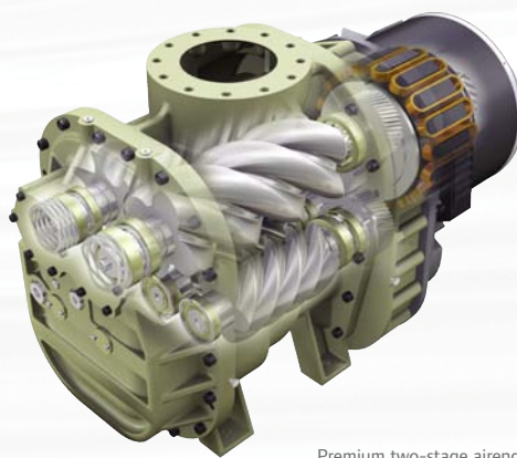
Premium two-stage air end
